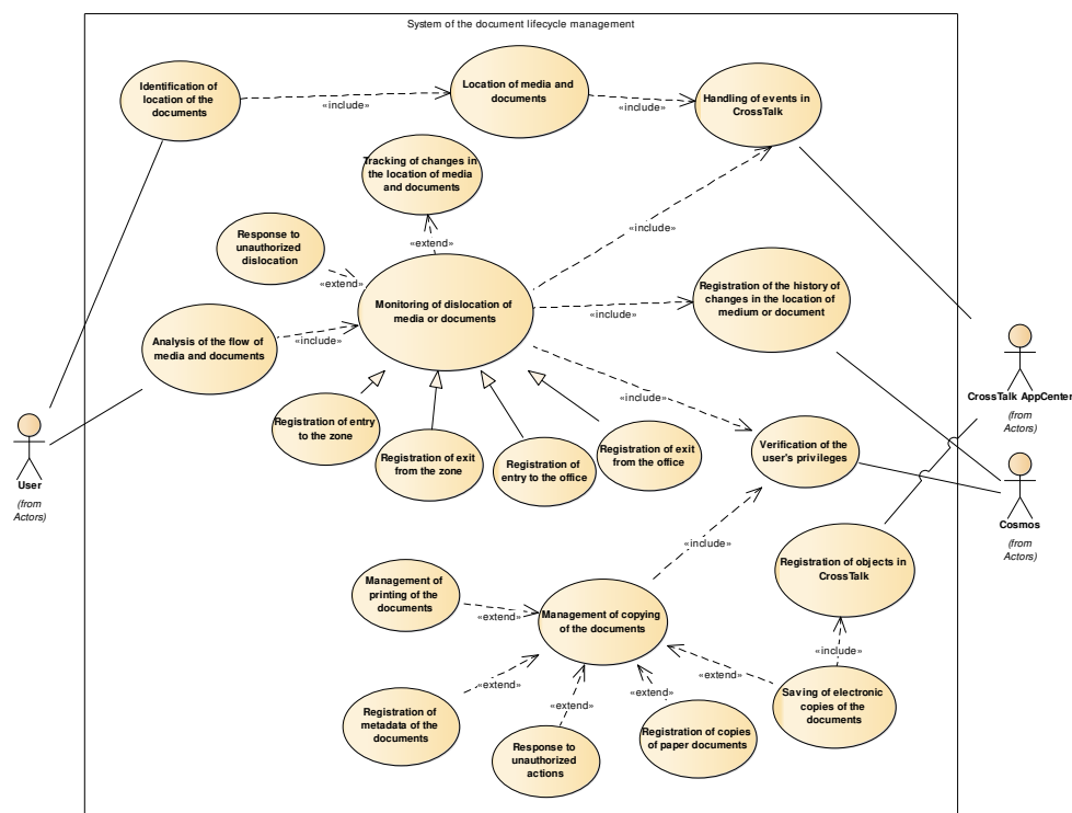
Fig. 4. Model of use cases
