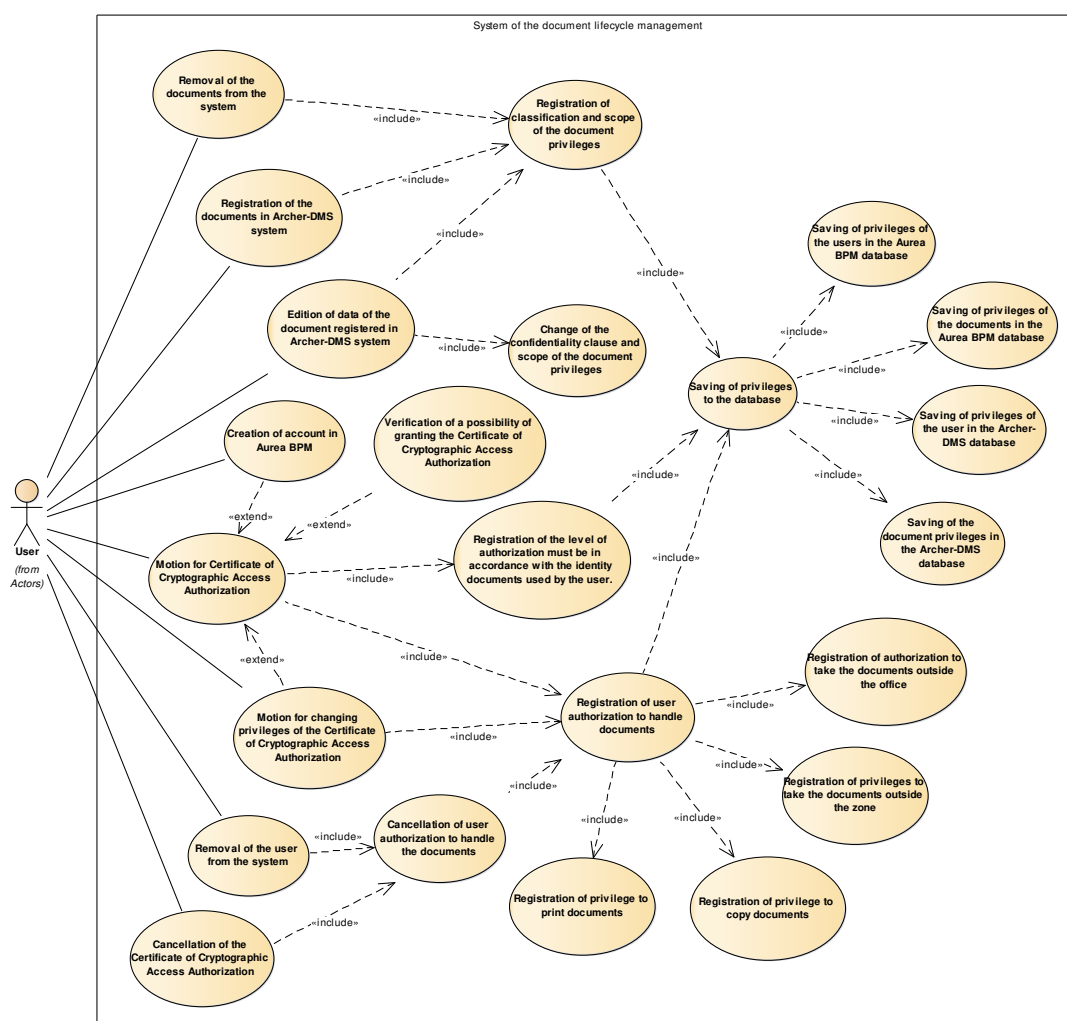
Fig. 5. Model of use cases
