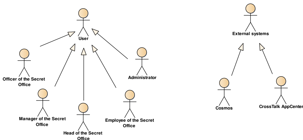
Fig. 3. System users
